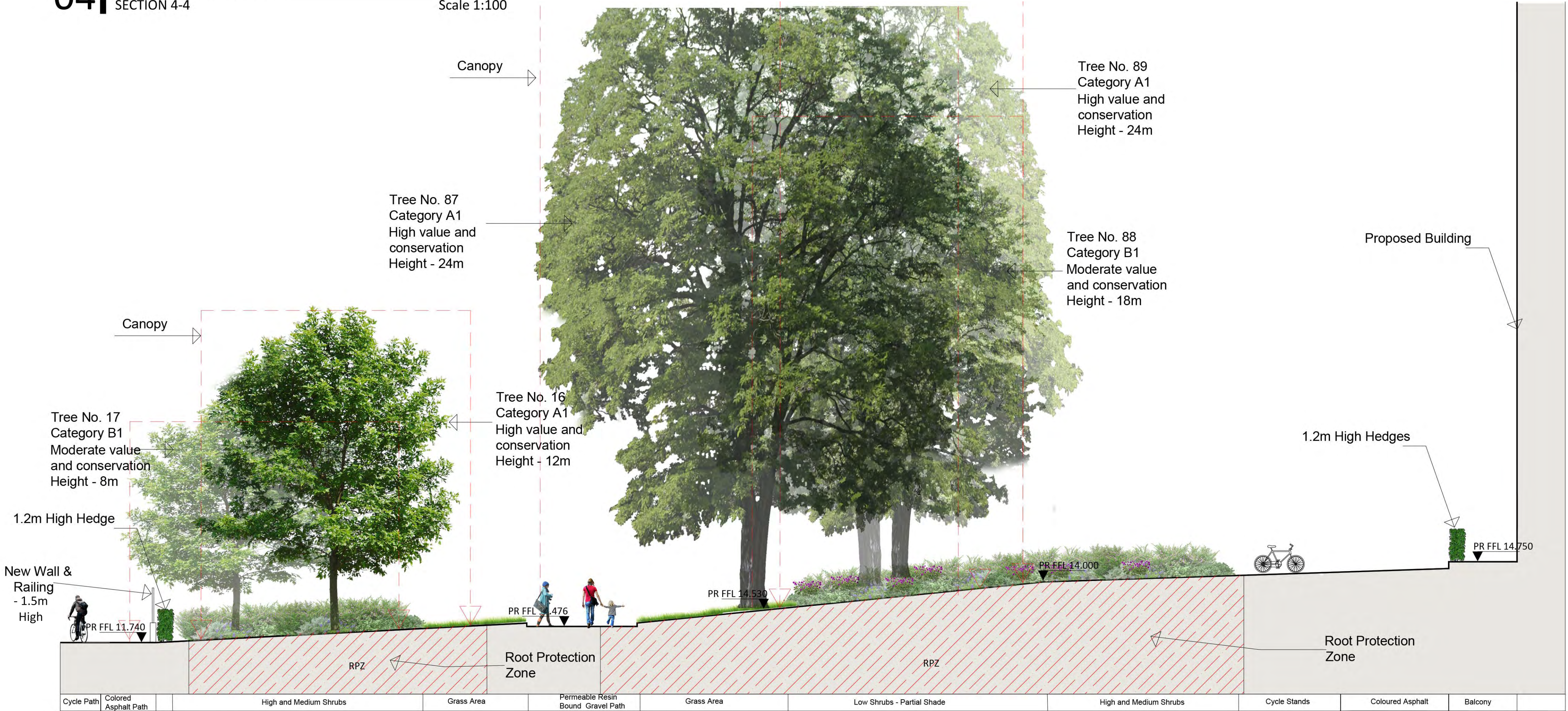
05 | Landscape Section SECTION 5-5
